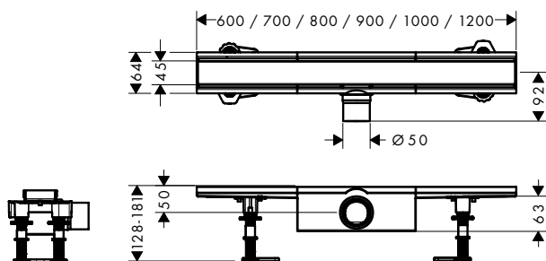
RainDrain Compact standardna instalacija
