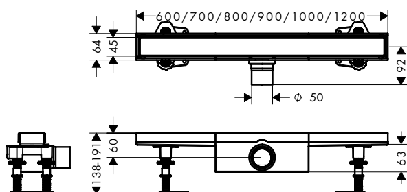
RainDrain Compact standardna instalacija
